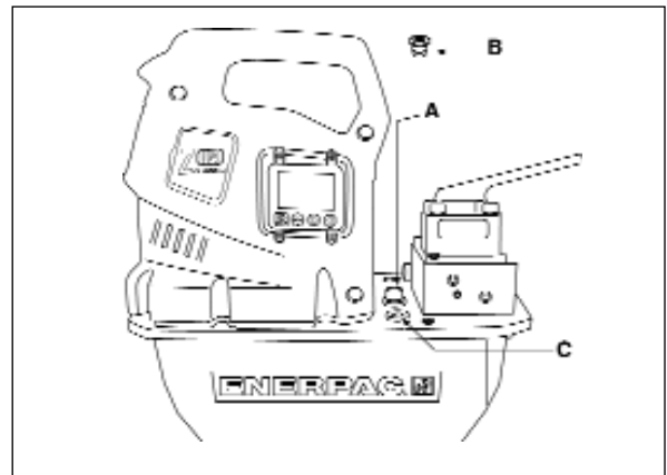
Figur 2, ZU4-ventilatormontering
