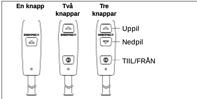
Figur 8, pendangknappens variationer
